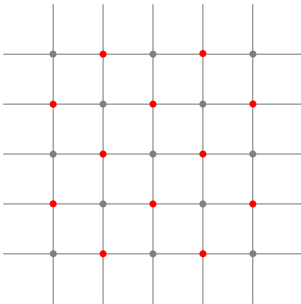
Figure 350: How the diamond-square algorithm works (5/5)
